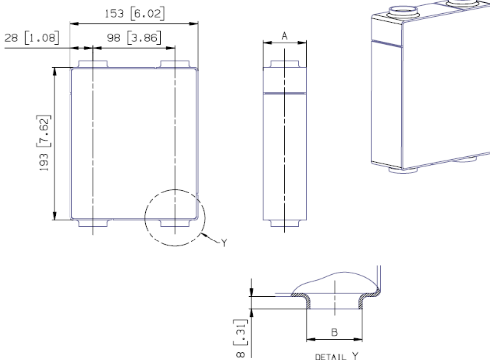
Dimensional Drawing mm (inches)
